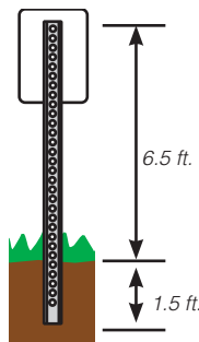
Closed Profile
